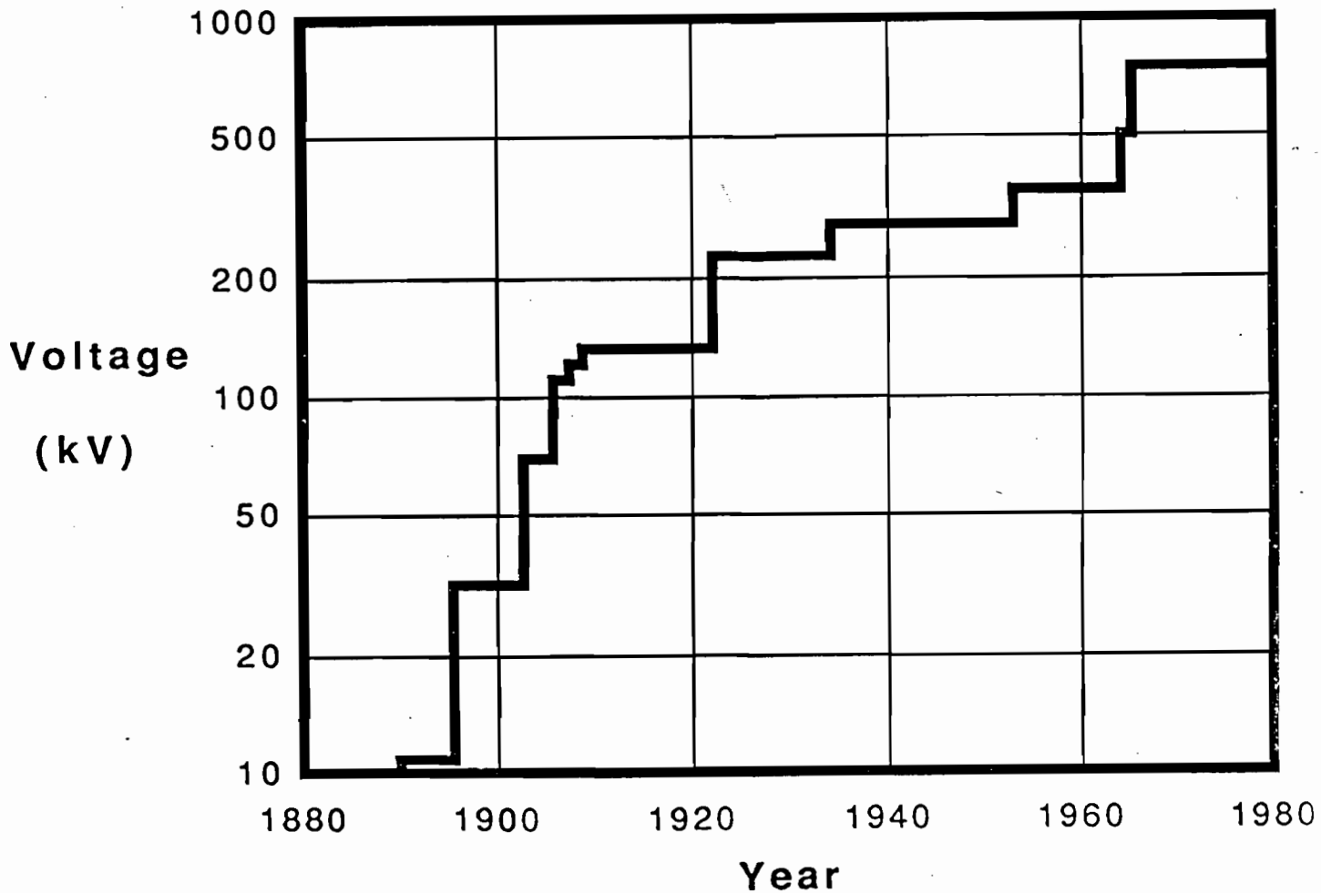
Figure 2-2: Highest 60 Hz transmission voltage in North America. From [Ellert 82].
