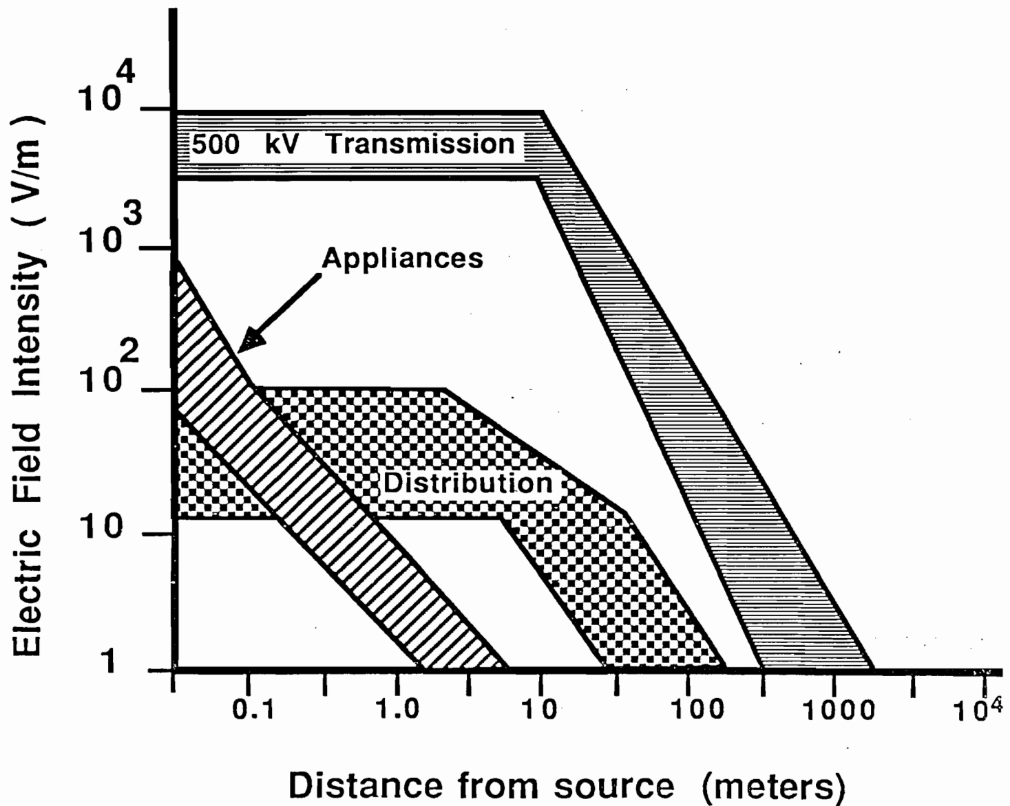
Figure 2-5: Illustration of how the electric field intensity at ground level changes with horizontal distance from three common sources of power-frequency electric fields. The bands represent variation across individual sources in each group. Adapted from [Florig 87a].
