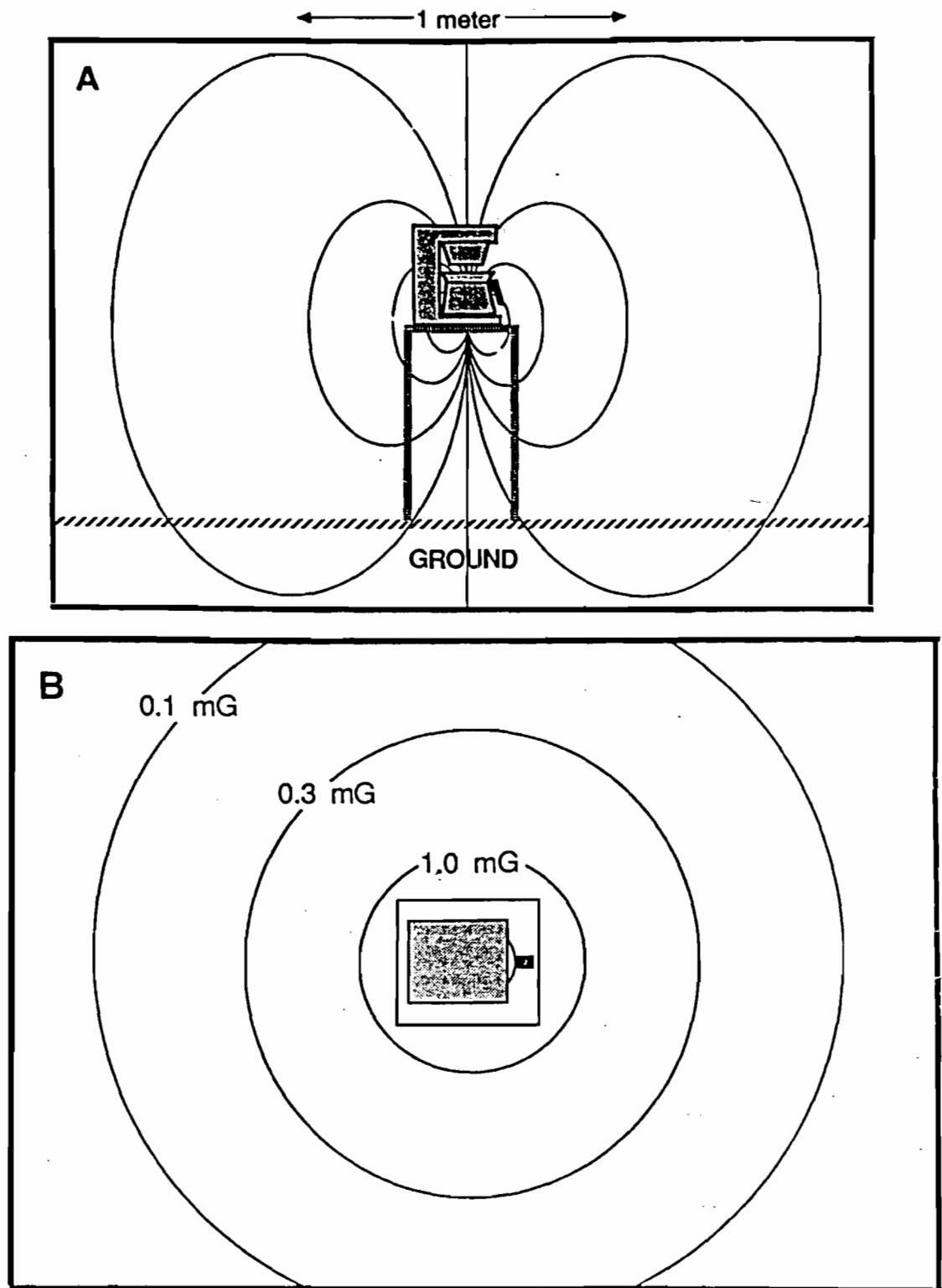
Figure 2-7: Time averaged (root mean square) magnetic field of a coffee maker (A) and top view (B) showing lines of equal flux density. Adapted from [Gauger 85].
